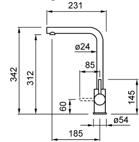
Technical Drawing
