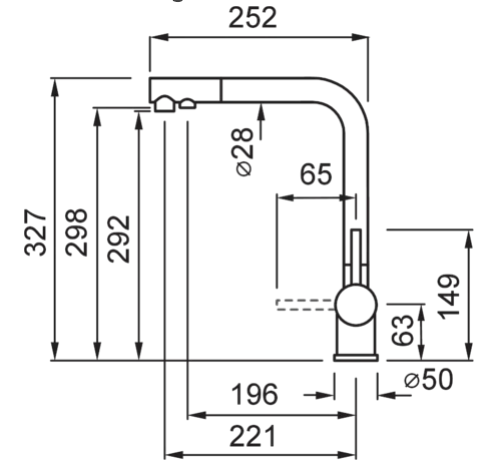
Technical Drawing
